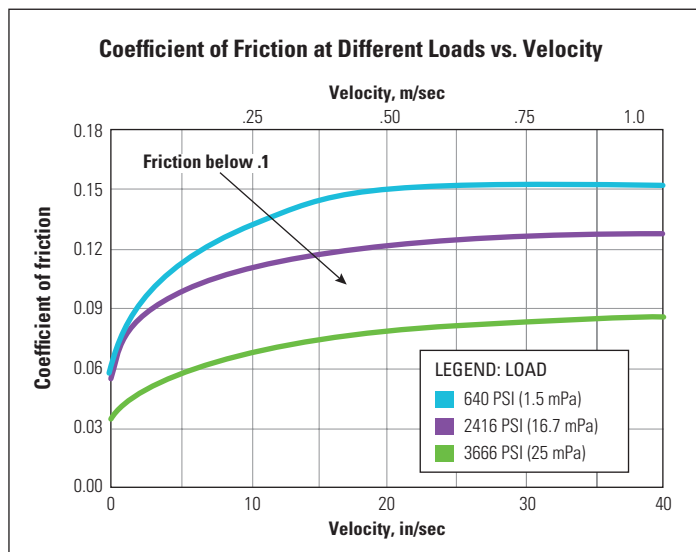
Figure 3. DuPont™ Vespel® CP-0664 Coefficient of Friction
