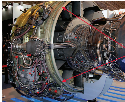
Figure 1. V-grooves are utilized in jet engine designs
