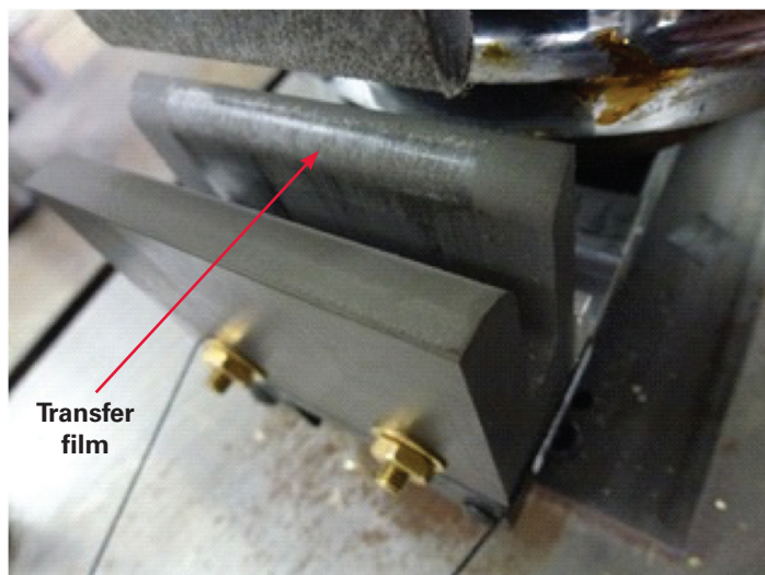
Figure 2. Impact/wear test fixture with transfer film on mating surface that reduces friction and enhances durability
